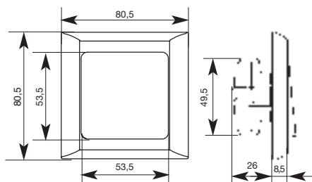
Intrerupator universal
